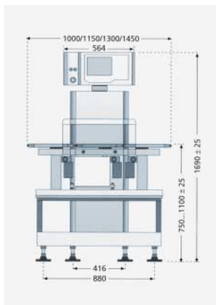
Scale drawing of EWK 1500 PLUS with WS 600 g, 1.25 kg and 6.0 kg
