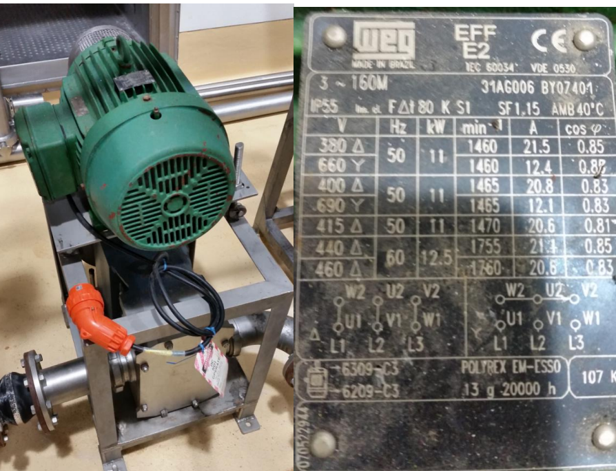
Coag transfer pump (lobe)
