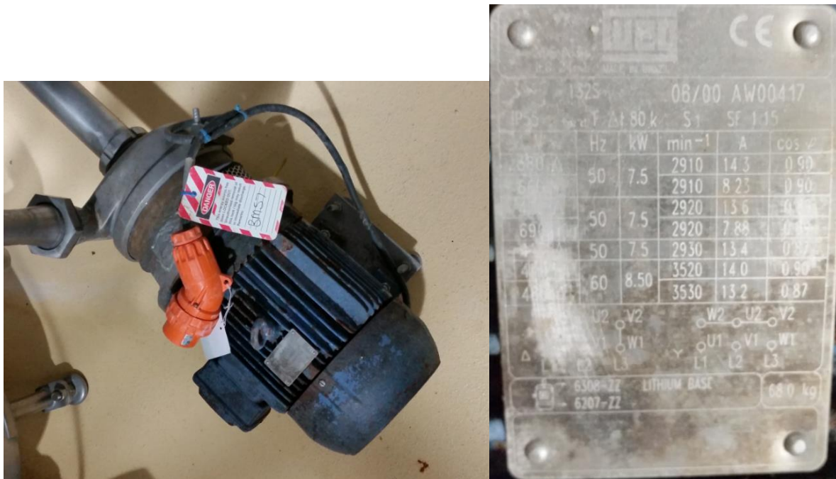
Centrifugal pump
